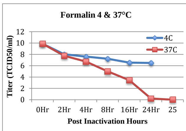
Figure-3. Inactivation of FMD virus serotype O with Formalin at 4°C & 37°C. Virus titers are presented as \log_{10}\text{TCID}_{50}/\text{ml} .
