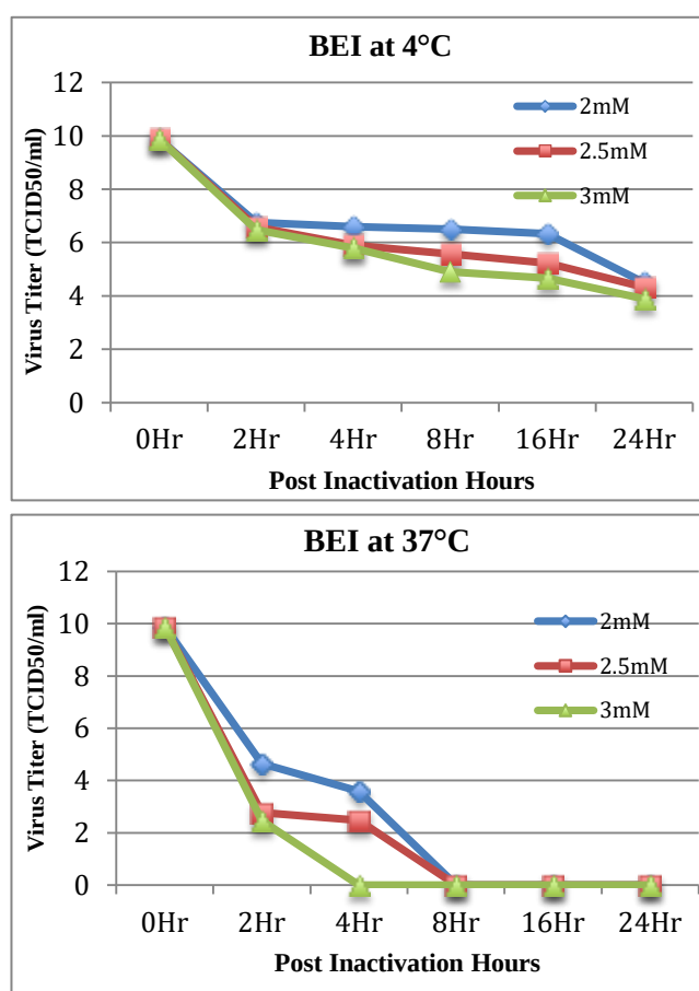
Figure-2. Inactivation of FMD virus serotype O with BEI at 4°C and 37°C. Virus titers are presented as \log_{10}\text{TCID}_{50}/\text{ml} .
