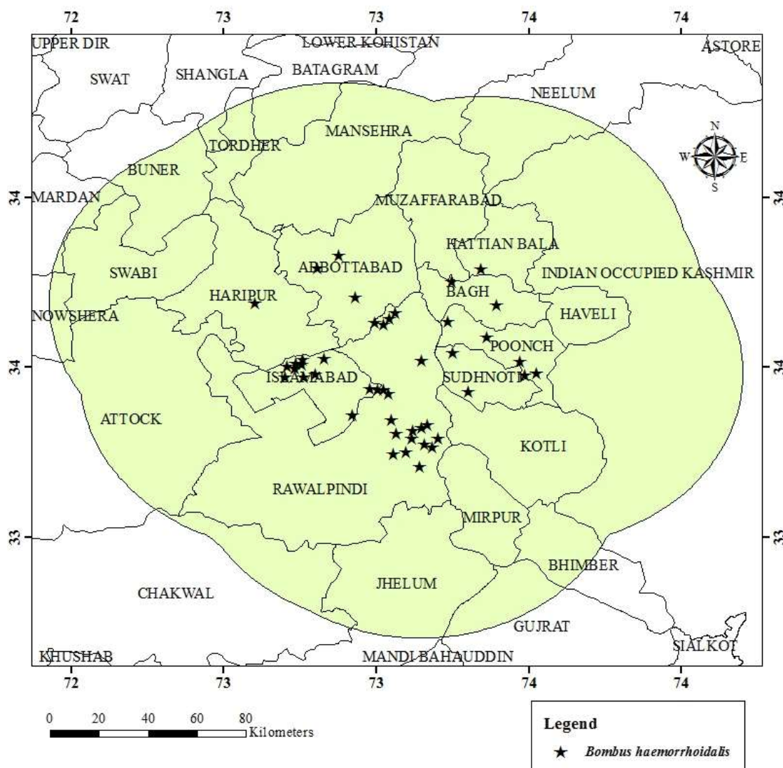
Figure-2. Occurrence points of the species along with buffer of 70 kilometers (M)
